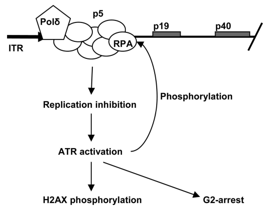
FIG. 8. Schematic representation of a model explaining how AAV2 provokes a DNA damage response. Pol \delta , DNA polymerase \delta .
